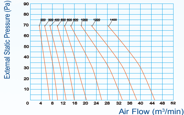
MKT3-200~1400G30
