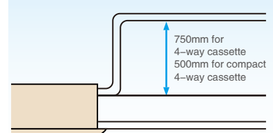
High water pump head
