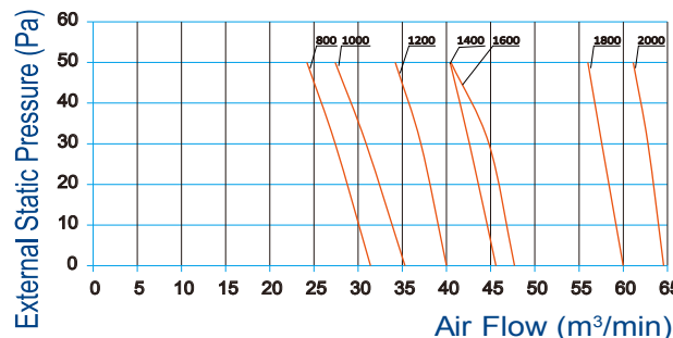
MKT4-800~2000G50-A4
