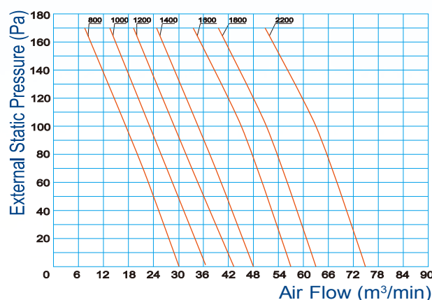
MKT3H-800~1400G70 MKT3H-1600~2200G100
