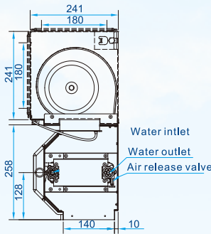
2-pipe duct
