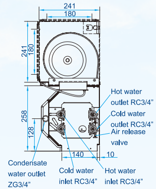
4-pipe duct
