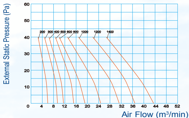
MKT3-200~1400G12
