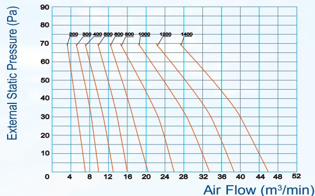
MKT3-200~1400G30
